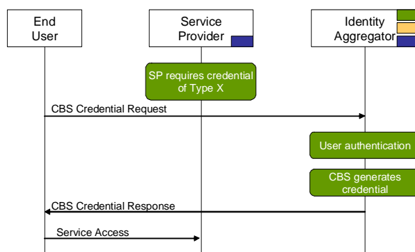
Figure 2: Credential bootstrapping service
