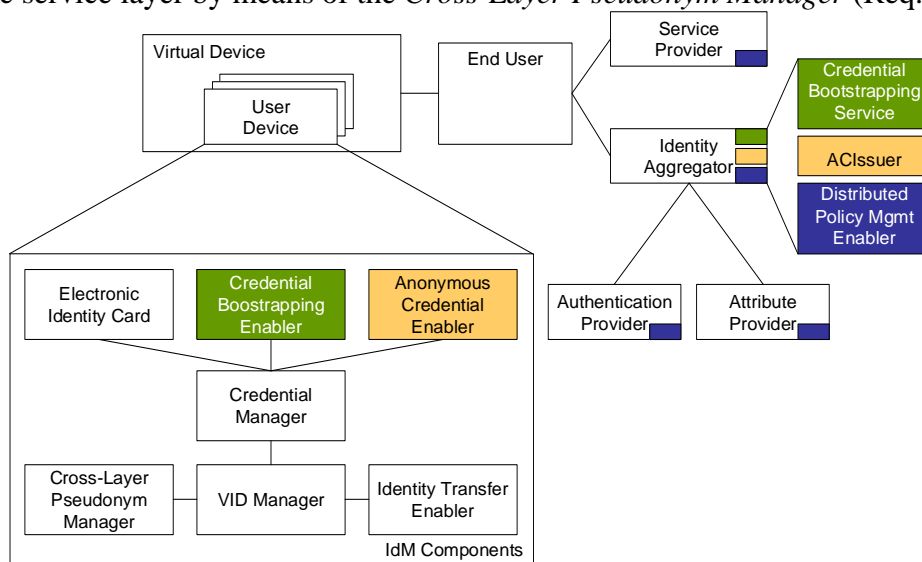
Figure 1: SWIFT Architecture
